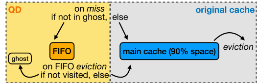
Figure 4: An example of QD: add a probationary FIFO queue to an existing cache.
